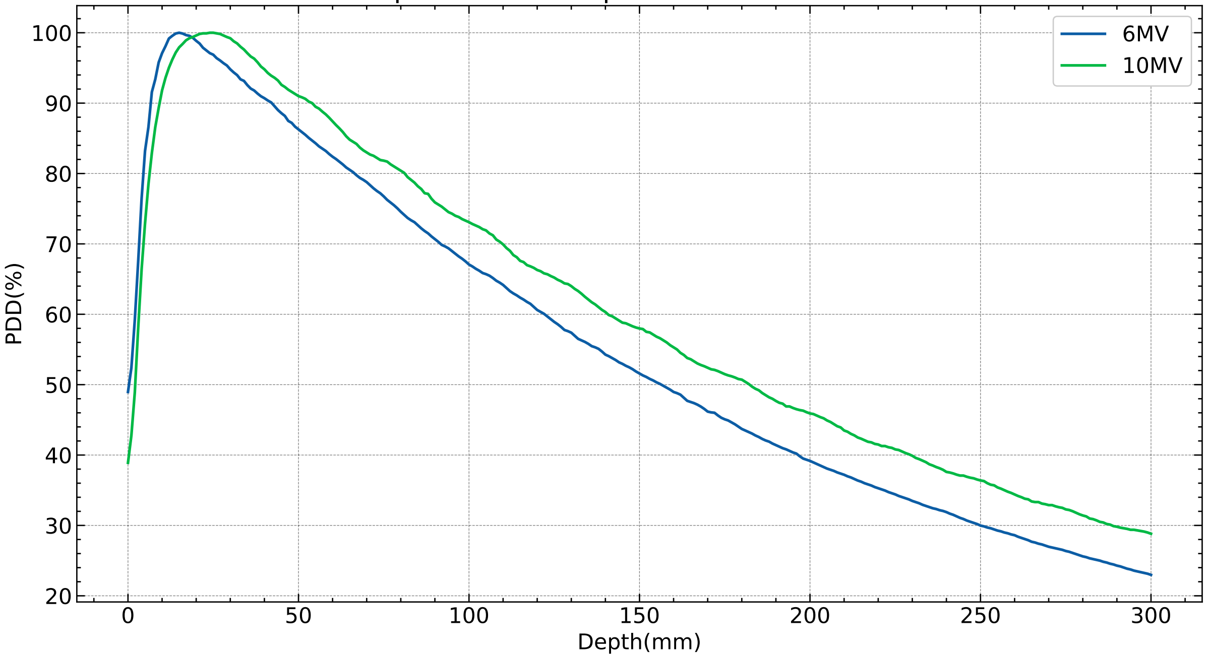
Comparison of PDD profiles of 6MV and 10MV
